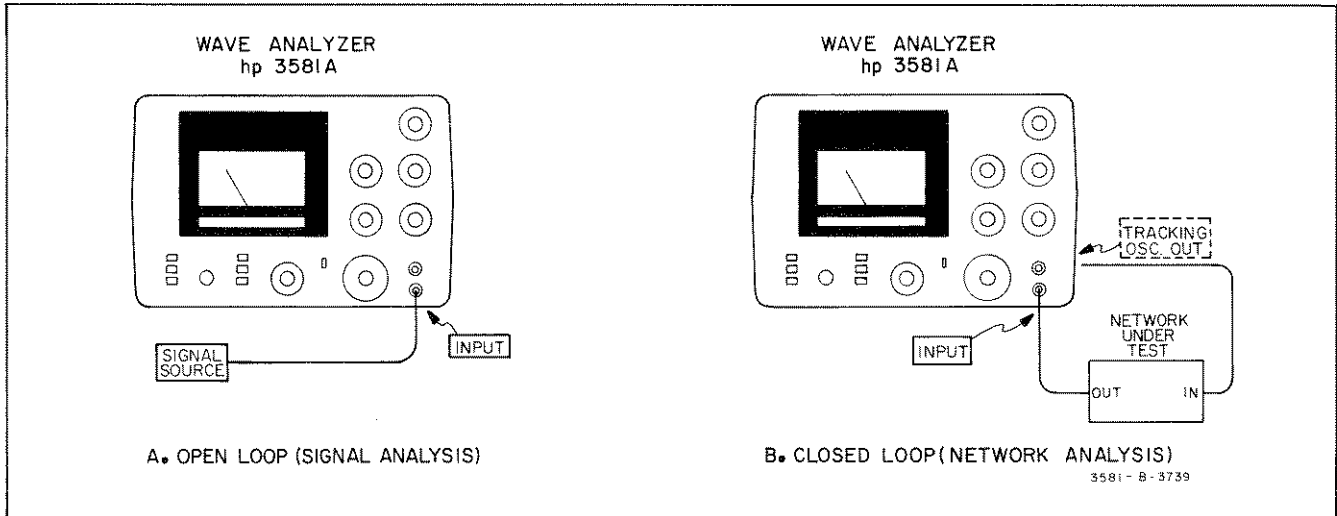
Figure 3-6. Measurement Configurations.
