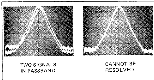
Figure 3-17. Two Signals in Passband.
