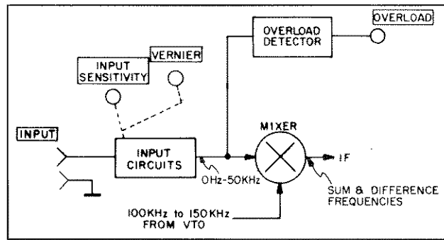
Figure 3-9. Input Section.
