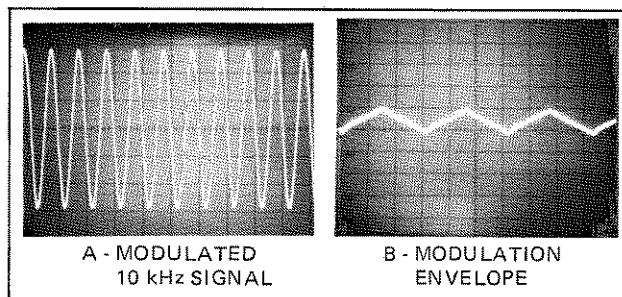
Figure 3-21. Amplitude vs. Time.
