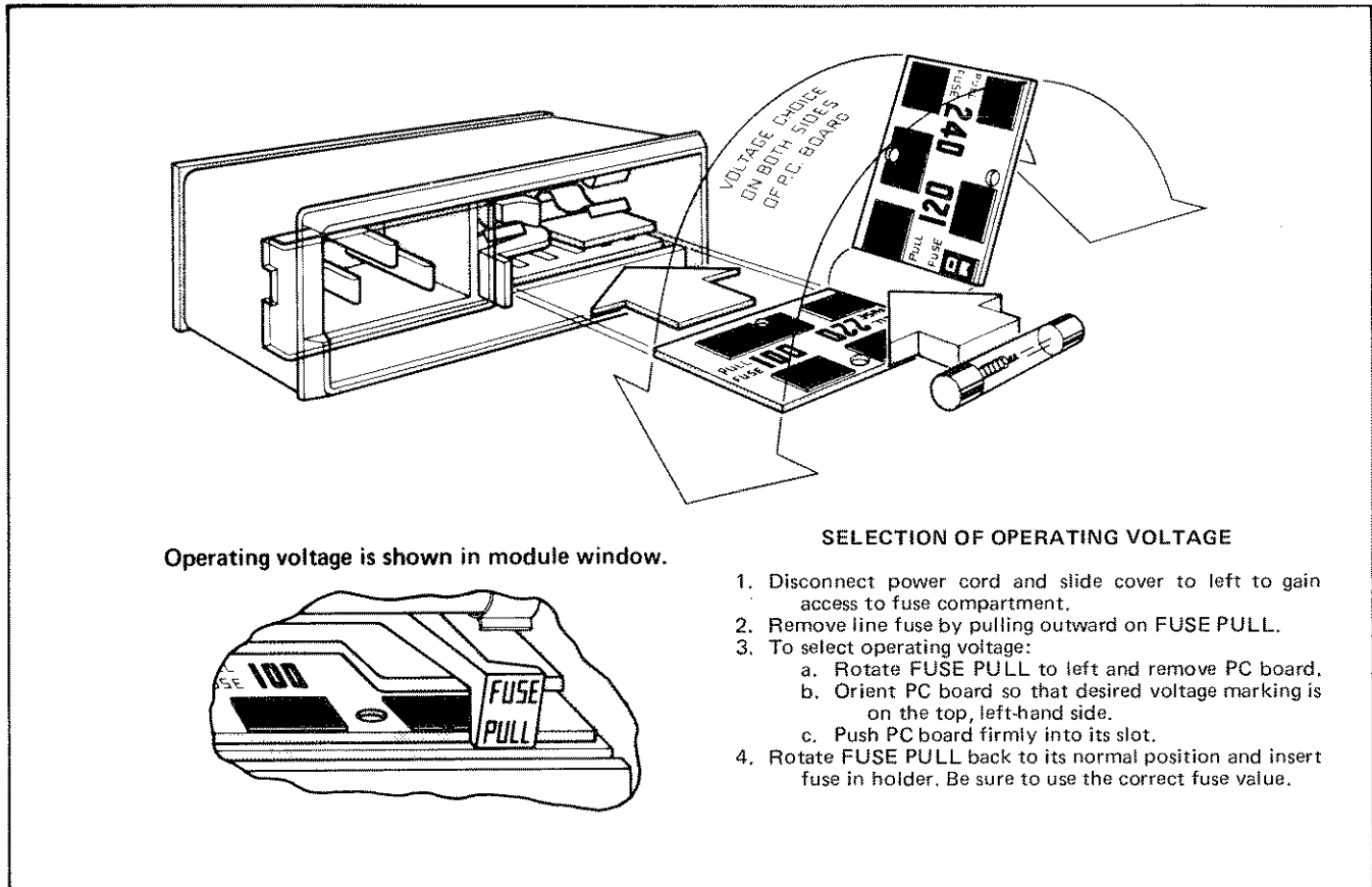
Figure 3-24. Voltage Selection.
